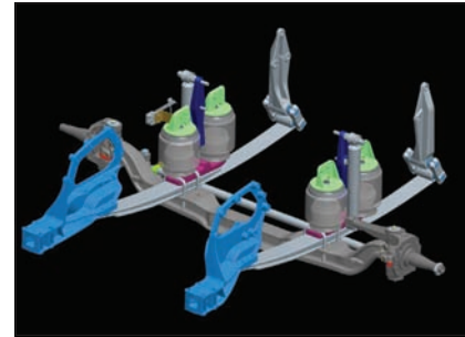
Peterbilt's proprietary new Front Air Leaf Suspension is lightweight and features a 20 percent improvement in ride quality over taper leaf suspensions for an extremely soft ride.
