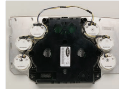
A multiplex electrical system offers diagnostic simplicity and reliability. The Electronic Service Analyst monitors the system, isolates sensors and gauges, and maintains an event log.
